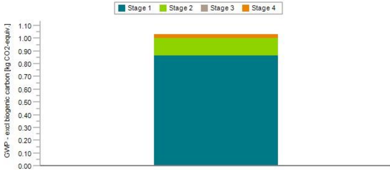
Figure 4: Global warming Potential, excluding biogenic carbon for design lifetime, (representative product, Behr PPUE 4850)
